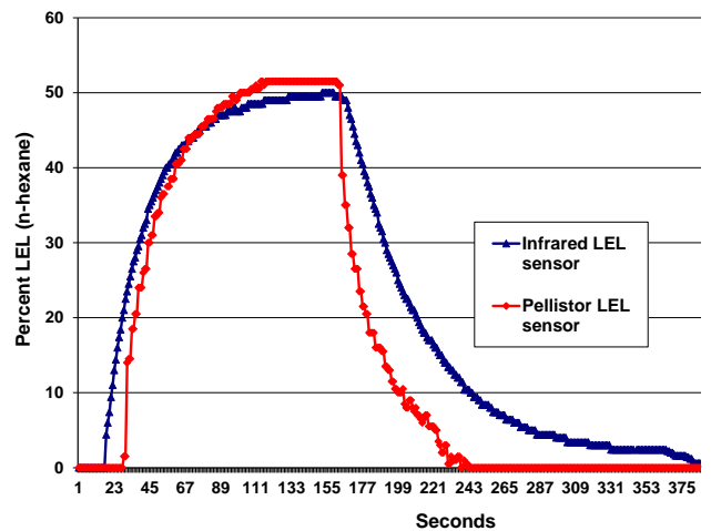
Figure 11: Response of n-hexane calibrated pellistor and IR sensors to 50% LEL n-hexane. The readings for both sensors are now very close to the true 50% LEL concentration applied. The initial response of the IR sensor is slightly quicker than the response of the pellistor sensor. However, the time to the final stable response (T100) is virtually identical for both sensors, (about 150 seconds).
