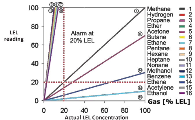
Figure 9: Two-wavelength infrared type LEL sensors usually measure combustible gas at a wavelength of 3.3 μm. The C-H bond in hydrocarbon molecules absorbs IR radiation at this wavelength. The more C-H bonds in the molecule, the greater the absorbance. As an example, in the attached graph the response to methane (CH 4 ), which has only four C-H bonds, is much lower than the response of the sensor to larger hydrocarbon molecules like pentane (C 5 H 12 ), which has 10 C-H bonds, or nonane (C 9 H 20 ), which has 20 C-H bonds.
