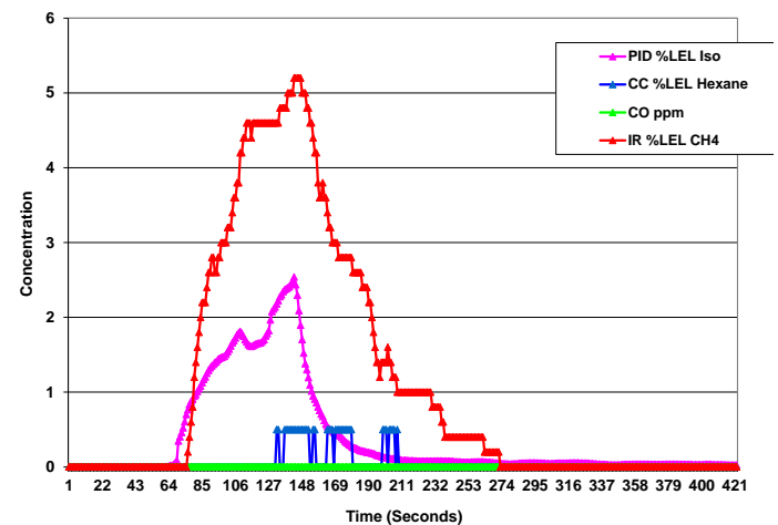
Figure 13: Response of PID, catalytic (pellistor) %LEL, IR %LEL and CO sensors exposed to diesel vapor. The IR LEL sensor shows the most accurate response, while the catalytic LEL sensor barely shows any response at all. PID is the best detection technology for low range ppm detection.
