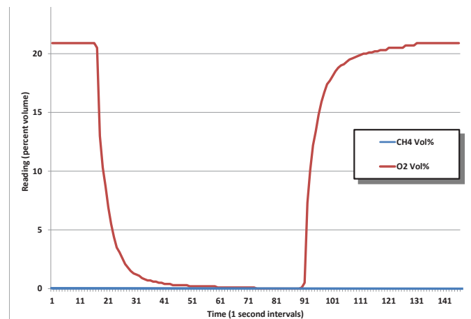
Figure 17: Response of infrared (IR) combustible gas and oxygen sensors exposed to 100% volume nitrogen (N 2 ). The IR combustible gas sensor showed no response when exposed to 100% volume nitrogen. The oxygen sensor rapidly dropped and stabilized on a reading of 0.0% volume when exposed to the N 2 test gas. The IR combustible gas sensor was set to the percent volume "HI Range" choice.
