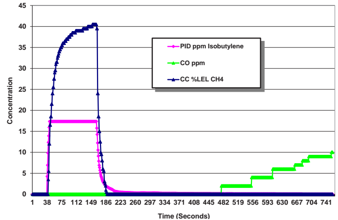
Figure 16: Response of standard pellistor (catalytic) LEL, O 2 , PID and CO sensors exposed to 50% LEL (9,000 ppm) isobutylene. The PID was calibrated to isobutylene. The LEL sensor was calibrated to methane (CH 4 ). The relative response of the LEL sensor to isobutylene is about 0.8. The maximum over-limit concentration of the PID is 1,700 ppm. Readings above this concentration are logged at this maximum value. Note the delayed response of the CO sensor to this very high concentration of VOC vapor.
