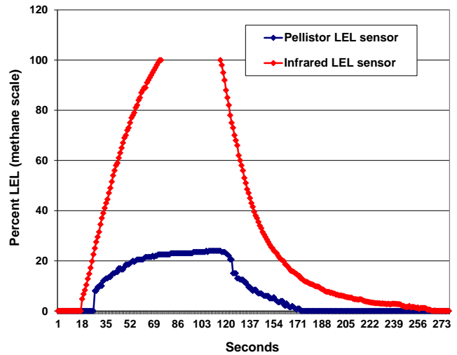
Figure 10: Relative response of pellistor and infrared sensors to n-hexane. Both sensors were calibrated to 50% LEL methane (CH 4 ), then exposed to 50% LEL n-hexane (C 6 H 14 ). The uncorrected readings for the pellistor sensor are much lower than the true concentration (50% LEL); while the uncorrected readings for the IR sensor are more than twice as high as the true concentration, (in fact, the readings exceeded the over-range limit of 100% LEL).
