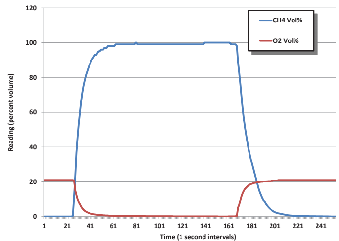
Figure 15: Response of "high range" (percent volume) infrared (IR) LEL and O 2 sensors exposed to 100% volume methane (CH 4 ). The IR combustible gas sensor was set to the percent volume "HI Range" choice. The IR combustible gas reading rapidly 100% volume CH 4 when exposed to 100% volume methane. The oxygen sensor rapidly dropped and stabilized on a reading of 0.0% volume when exposed to the oxygen free CH 4 gas.
