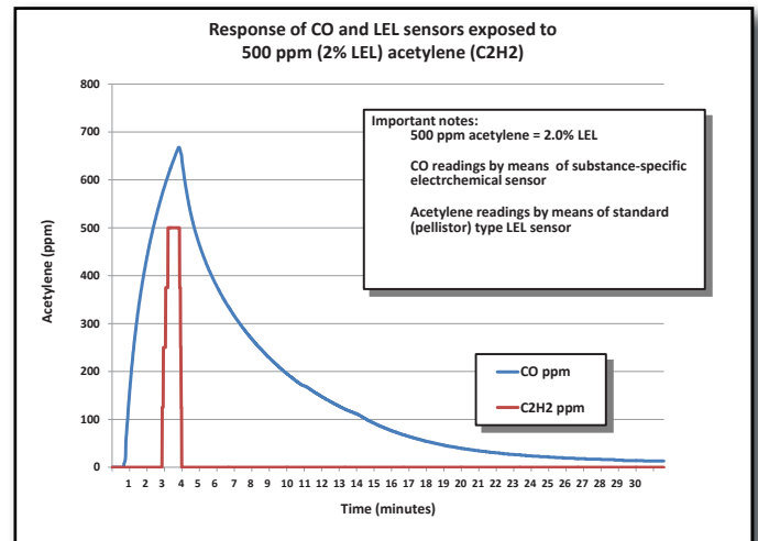
Figure 3: Electrochemical CO sensors can take a long time to clear after exposure to certain interfering contaminants such as acetylene.
