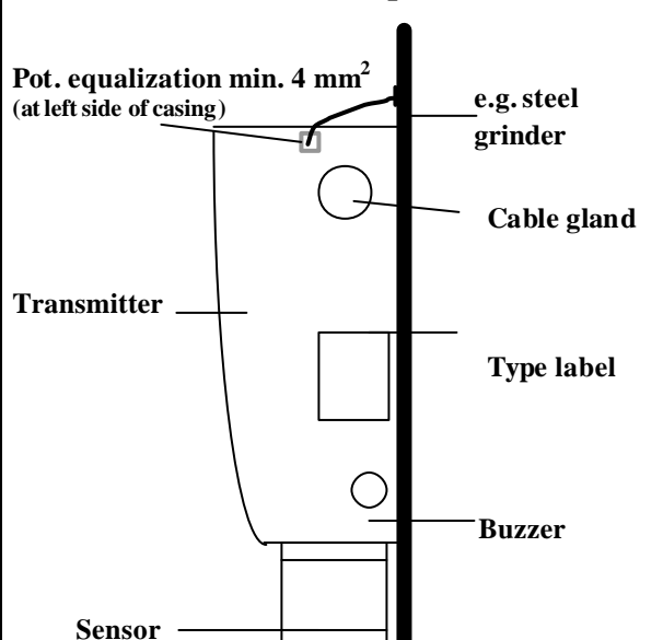
Potential equalization
