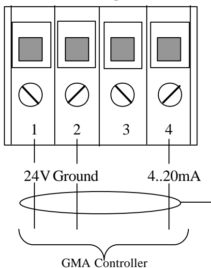
Terminal diagram
